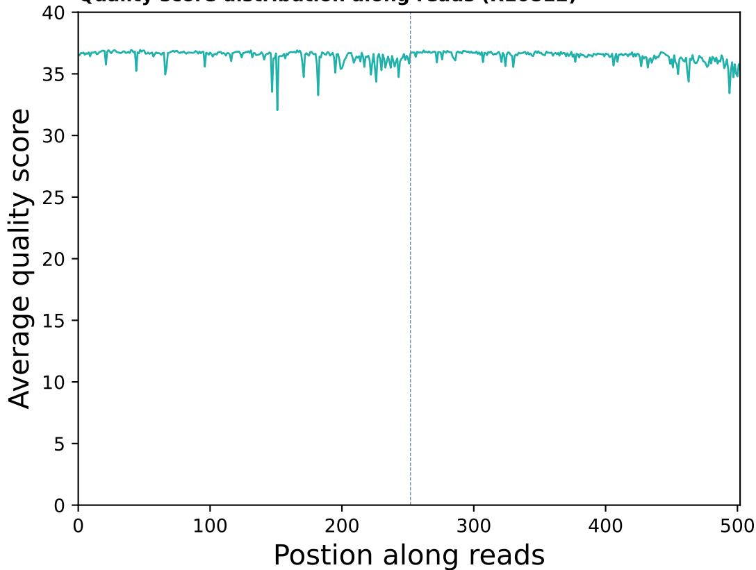
Quality score distribution along reads (R10812)
